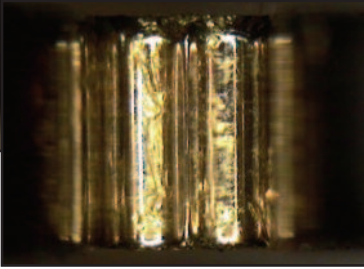
Gross Deformation of Crimped Terminal Resulting from Material Buildup in Crimper
