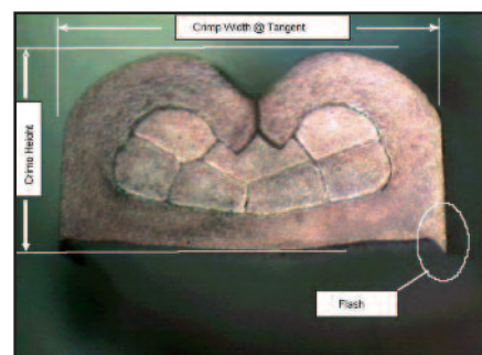
Cross Section Defining Crimp Width, Crimp Height, and Flash
