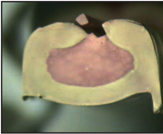
Visible Deformation of Outer Crimp Surface as a result of Indentation from Material Buildup on Crimper
