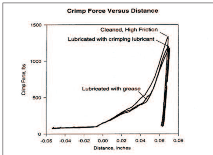
Typical Effect of Friction on Crimp Force
